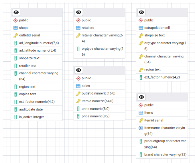
Fig 4. ERD of Panel IMS DB generated by pgAdmin
