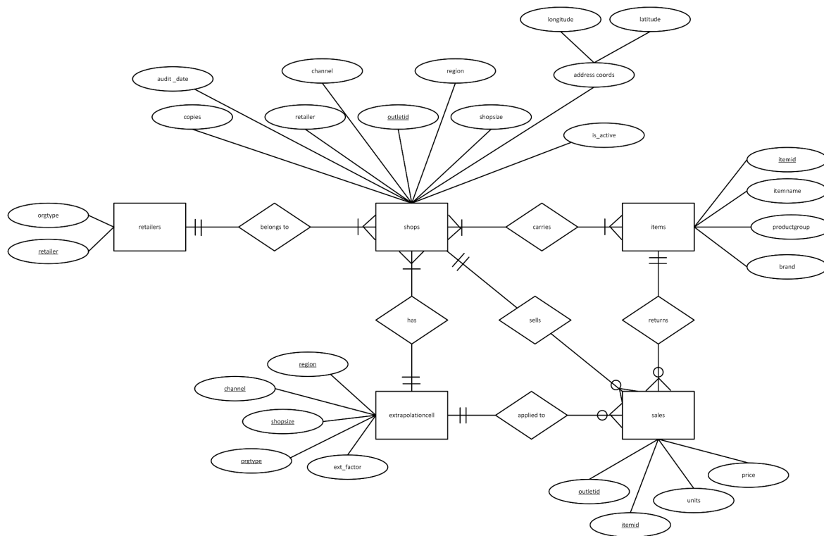
Fig 2. ERD of Panel IMS
